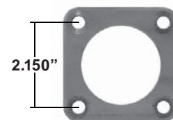
Greddy 47 mm
